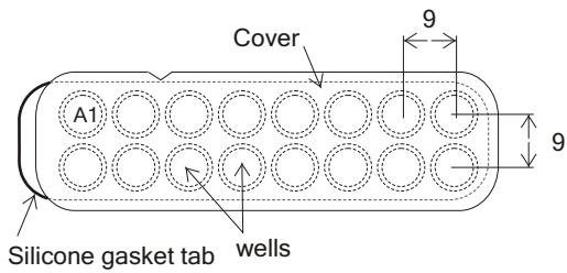
Top View of Assembled Unit
